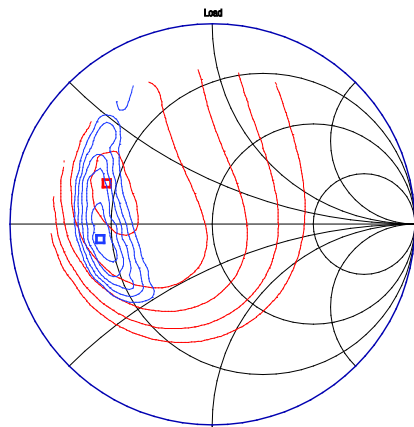
Figure 19. OIP3 Load Pull @ 0.75 GHz, 5 V, 76 mA (Input Load = NF Min., -20 dBm/Tone, 5 MHz Spacing)
