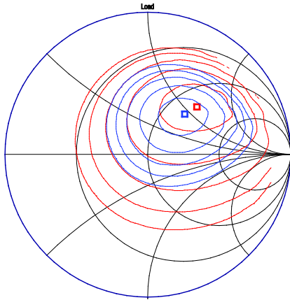
Figure 17. OIP3 Load Pull @ 0.35 GHz, 5 V, 76 mA (Input Load = NF Min., -20 dBm/Tone, 5 MHz Spacing)
