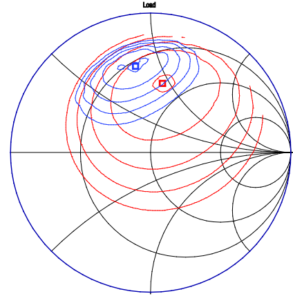
Figure 18. OIP3 Load Pull @ 0.45 GHz, 5 V, 76 mA (Input Load = NF Min., -20 dBm/Tone, 5 MHz Spacing)
