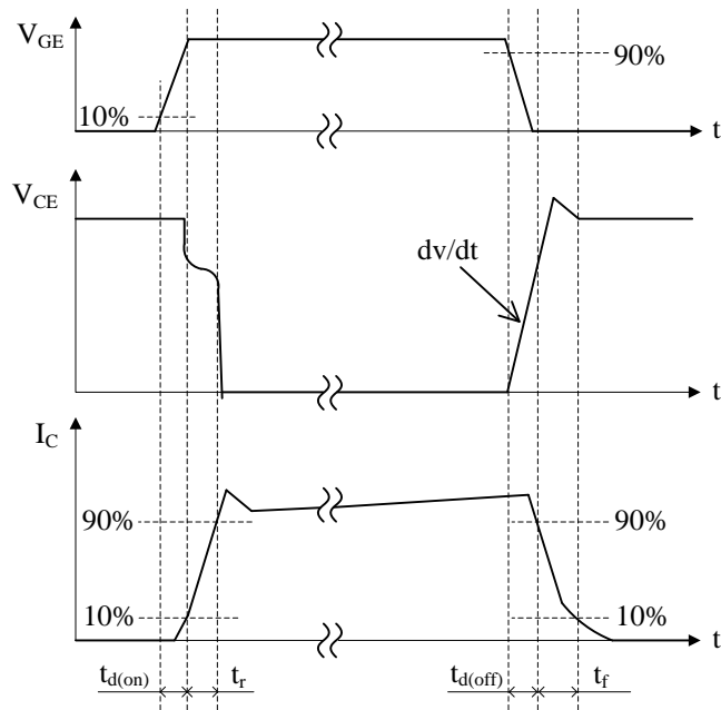
Figure 1 Test Circuits and waveforms of dv/dt and Switching Time
