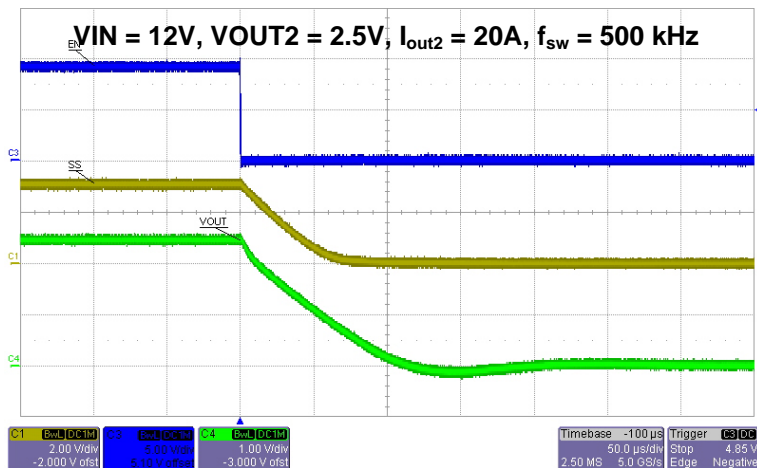
Fig. 8 Channel-2 Power Down Sequence (C3: EN, C1: SS2, C4: VOUT2)
