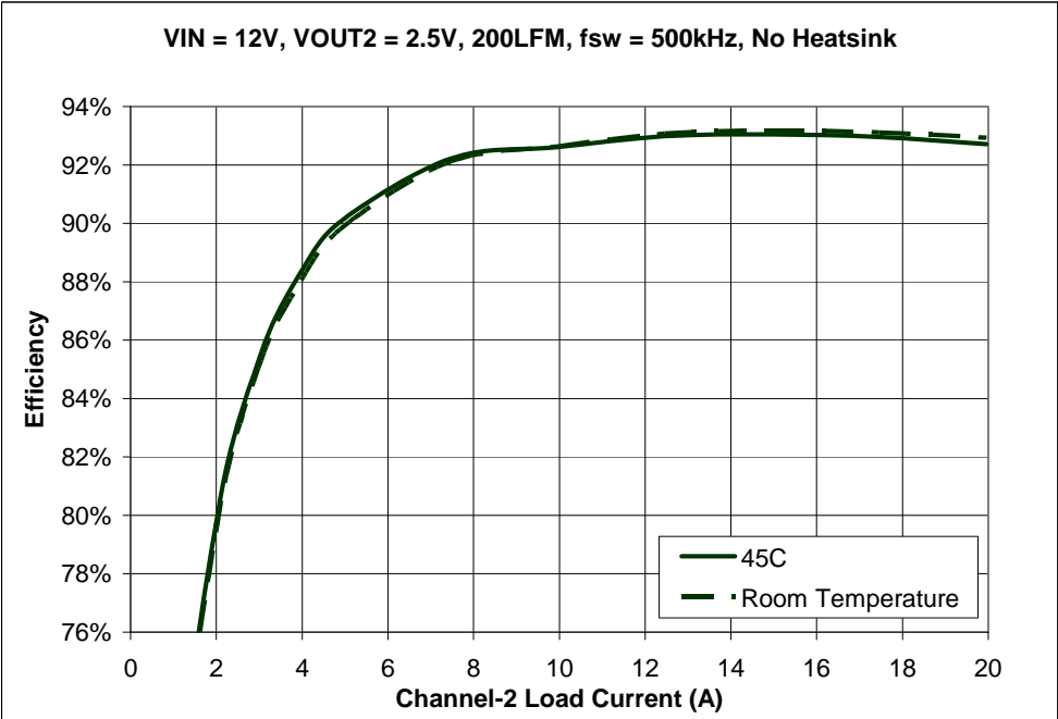
Fig. 23 Channel-2 Efficiency
