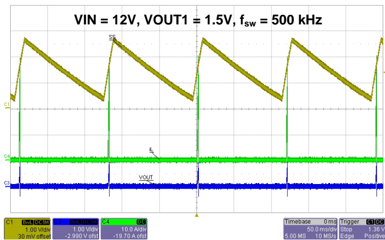
Fig. 9 Hiccup Mode Over Current Protection (C1: SS1, C4: I out1 , C3: VOUT1)
